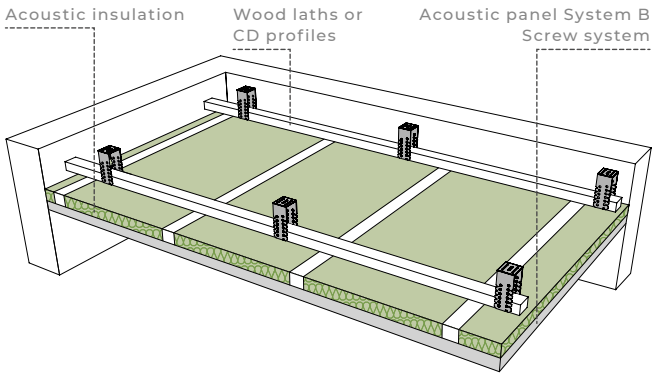
Recommended structure for wood wool acoustic panels on wooden laths or CD profiles with insulation layer ISOLENA Optimal Plus
